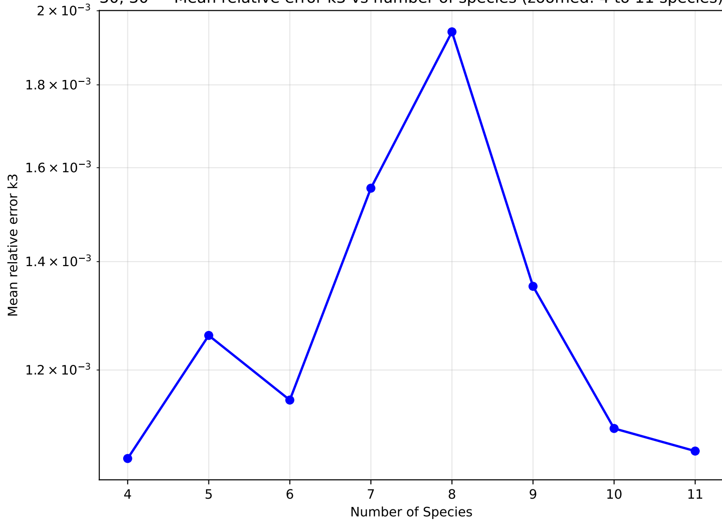
30, 30 — Mean relative error k3 vs number of species (zoomed: 4 to 11 species)
